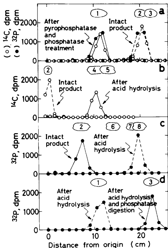
Fig. 2. Identification of the product of galactosyl-phosphotransferase: (a) paper electrophoretogram of the ^{14}\text{C} -labeled product (○) and ^{32}\text{P} -labeled product (●), before (-----) or after (—) treatment with nucleotide pyrophosphatase and alkaline phosphatase (fig. 1, reactions 1 and 2); (b) paper chromatogram in solvent B of the ^{14}\text{C} -labeled product, before (-----) or after (—) mild acid hydrolysis (fig. 1, reaction 3); (c) paper chromatogram in solvent A of the ^{32}\text{P} -labeled product, before (—) or after (-----) mild acid hydrolysis (fig. 1, reaction 3); (d) paper electrophoretogram of the acid hydrolysate of ^{32}\text{P} -labeled product, before (-----) or after (—) treatment with alkaline phosphatase (fig. 1, reaction 4). See [2] for details of the procedure. Standards: 1, GlcNAc-P-Gal; 2, UDP-GlcNAc-P-Gal; 3, inorganic phosphate; 4, galactose; 5, glucose; 6, UDP; 7, UMP; 8, GlcNAc-6-P.
